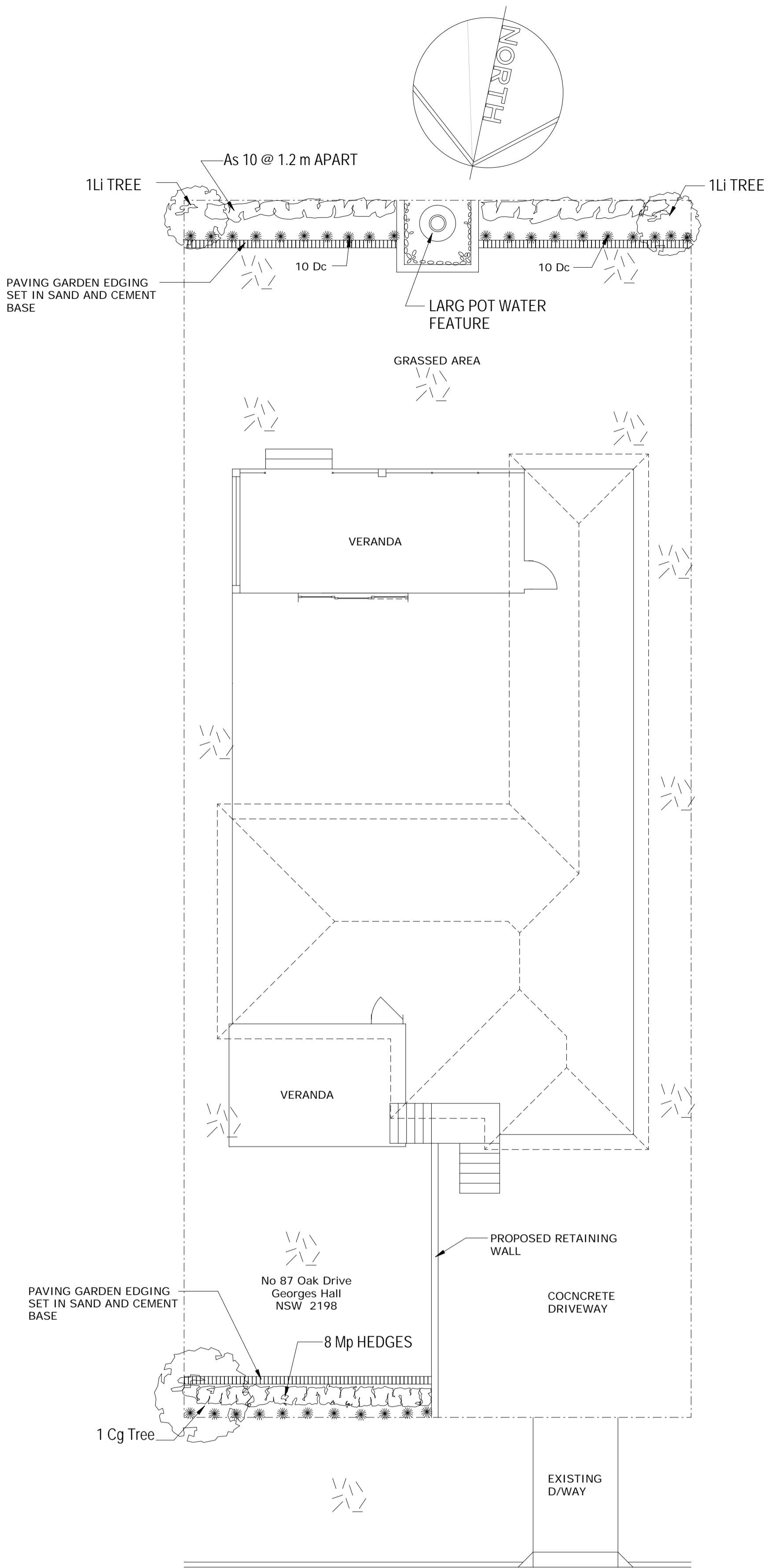
CONCEPT LANDSCAPE PLAN Scale 1 :100
